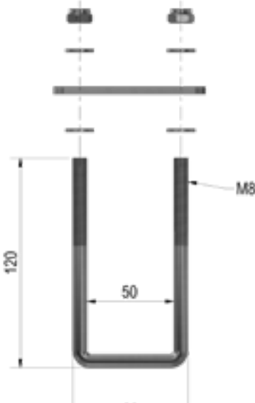
With this mounting set is it possible to mount a box on a drawbar.
